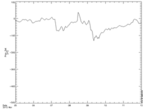
Numerical Data Geomagnetic Equatorial Dst Index Provisional
