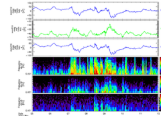
Numerical Data MM210 Kototabang magnetometer 1 min resolution data distributed by ERG-SC
