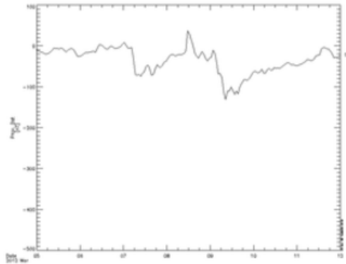
Numerical Data Geomagnetic Equatorial Dst Index Provisional
