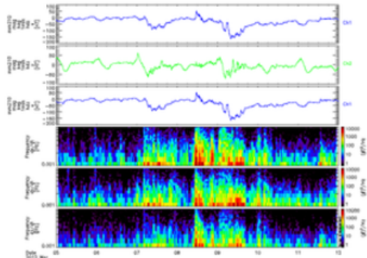
Numerical Data MM210 Kagoshima magnetometer 1 min resolution data distributed by ERG-SC
