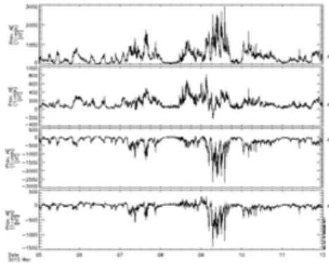
Numerical Data Geomagnetic Auroral Electrojet Index Provisional AE
